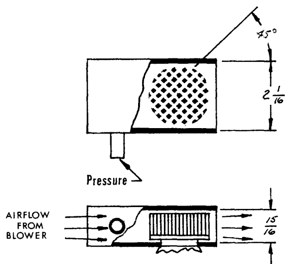
- COWLING DETAIL -
