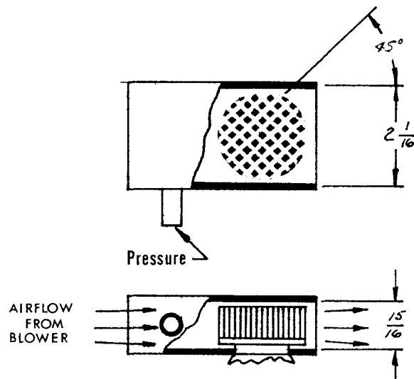
- COWLING DETAIL -
