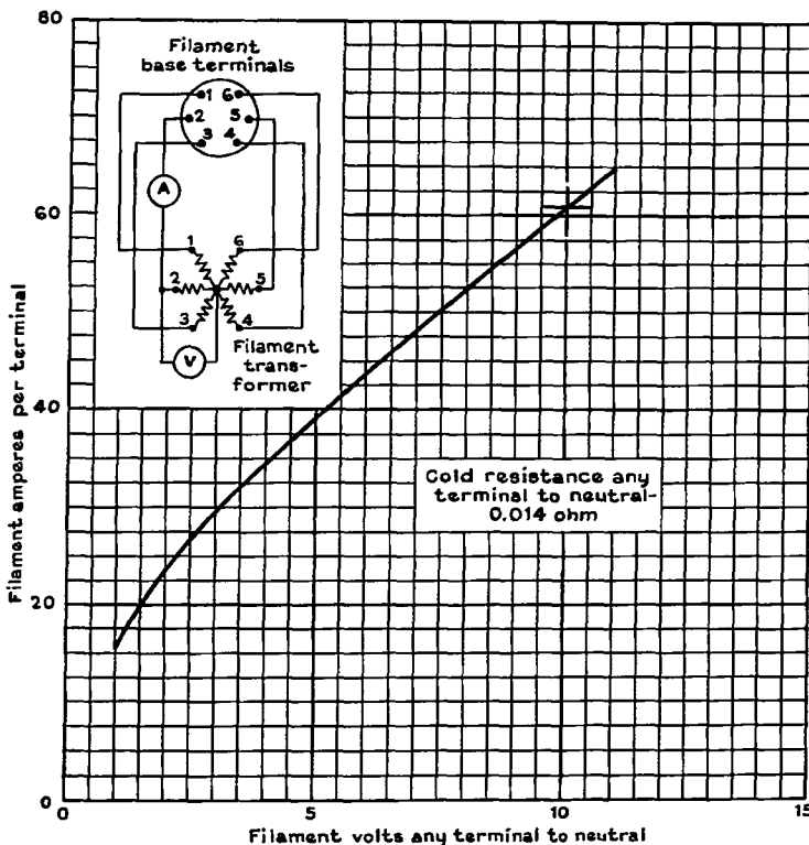
Average Filament Characteristic K-7050605 5-22-39
