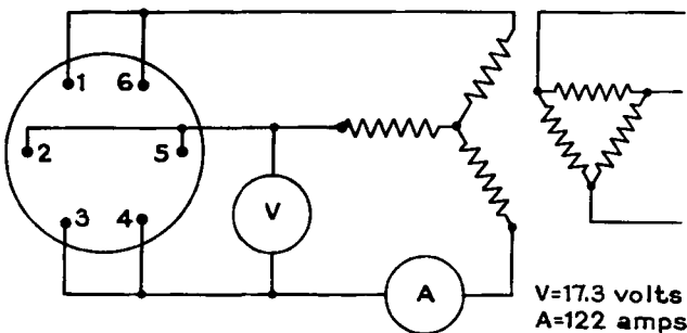
Three-phase A-c Filament Excitation
