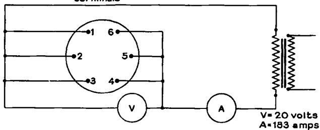
Single-phase A-c Filament Excitation
