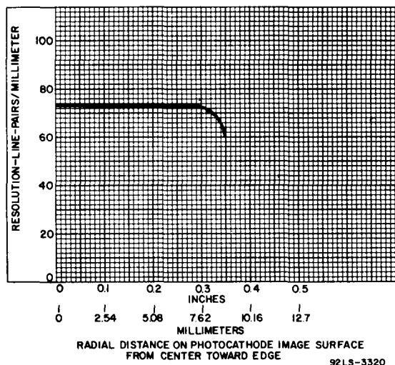
TYPICAL RESOLUTION AS A FUNCTION OF RADIAL DISTANCE ON PHOTOCATHODE FOR TYPES 8857/V1, 8857/V2
