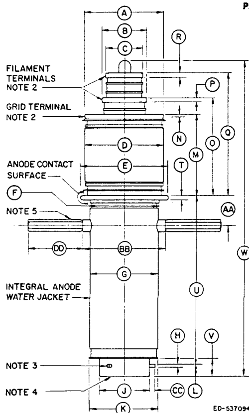
OUTLINE OF ML-8795
