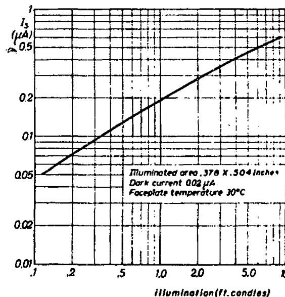
Figure 6. Average Signal Current vs. Illumination on the Photoconductive Layer
