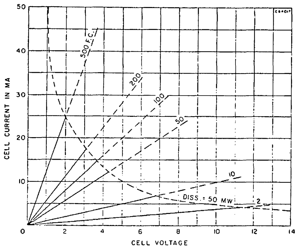
CELL CURRENT AND DISSIPATION VS VOLTAGE
