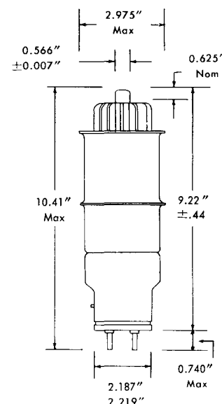
OUTLINE DRAWING
