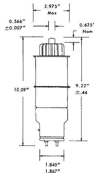
OUTLINE DRAWING
