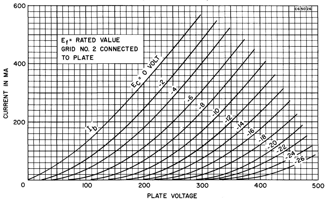
AVERAGE PLATE CHARACTERISTICS (Triode Connected)
