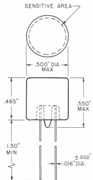
OUTLINE 8346
