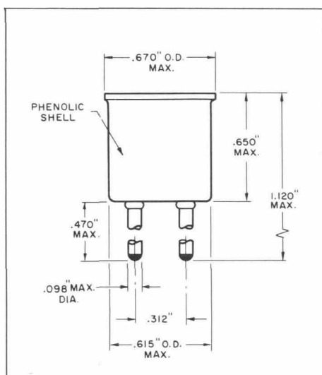
OUTLINE 8346-1
