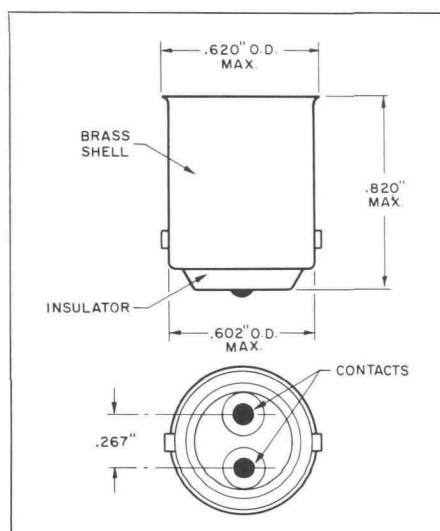
OUTLINE 8346-7
