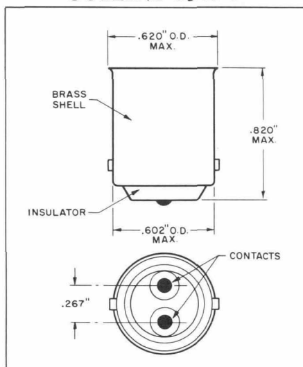
OUTLINE 8345-7
