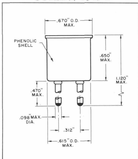
OUTLINE 8345-1
