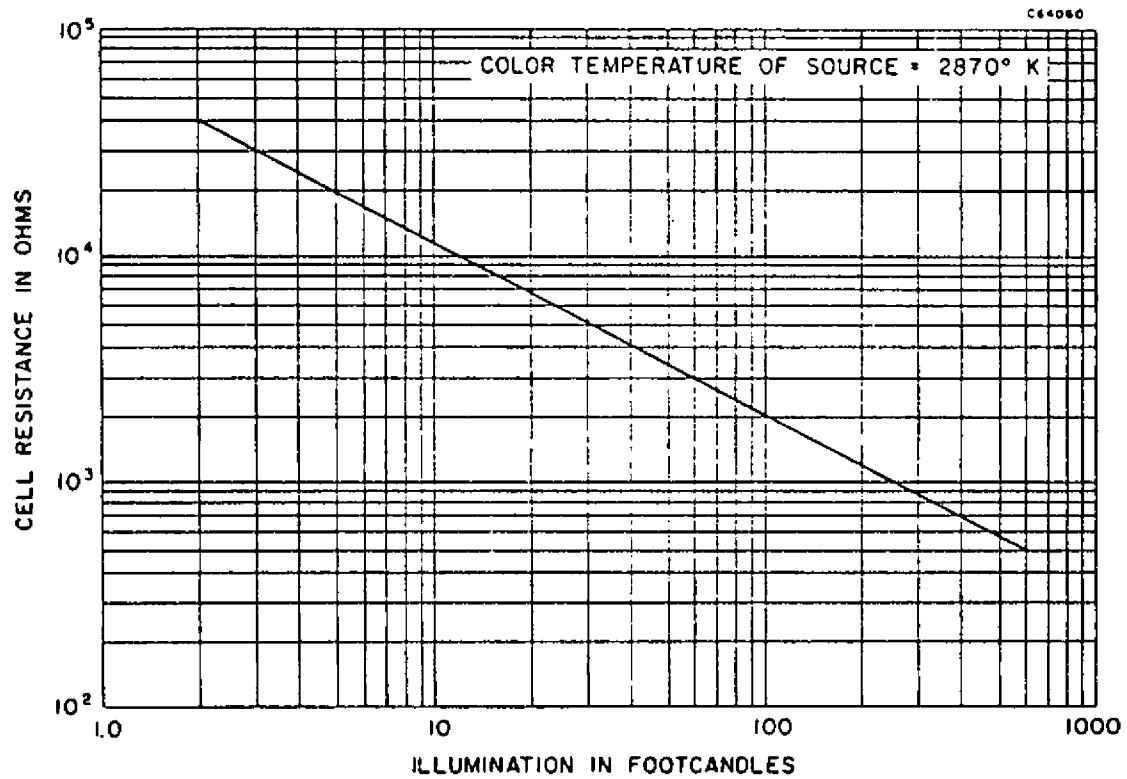
CELL RESISTANCE VS ILLUMINATION
