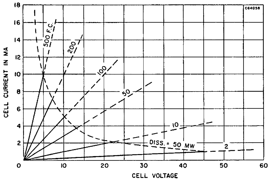
CELL CURRENT AND DISSIPATION VS VOLTAGE
