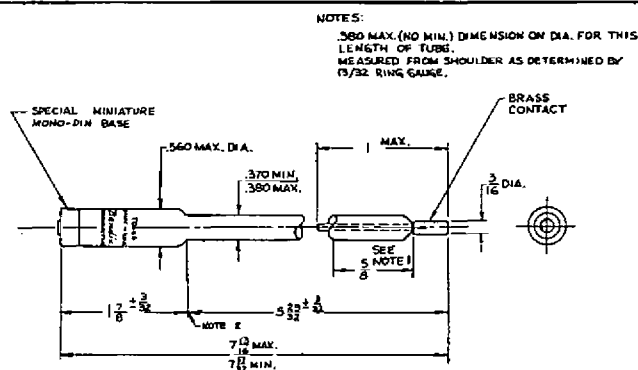
OUTLINE DRAWING
