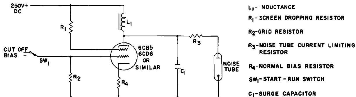
FIGURE 1. BASIC STARTING AND OPERATING CIRCUIT
