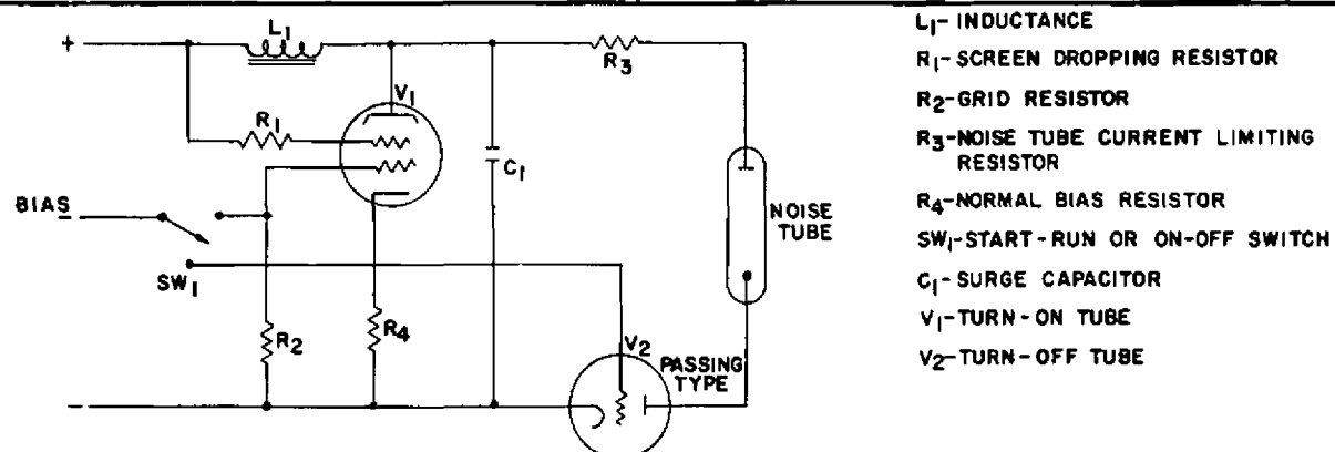
FIGURE 2 PULSED STARTING AND OPERATING CIRCUIT
