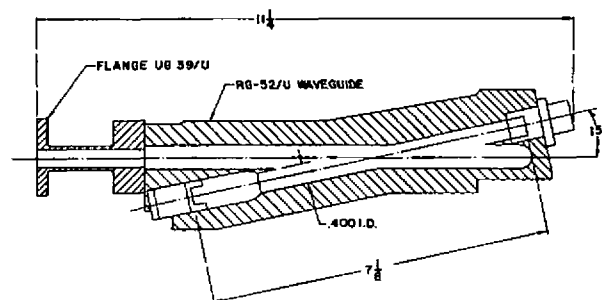
TERMINATED 15° WAVEGUIDE MOUNT ASSEMBLY
