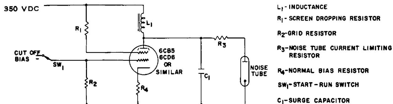
FIGURE 1. BASIC STARTING AND OPERATING CIRCUIT
