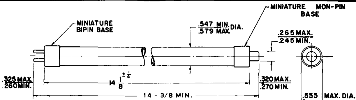
OUTLINE DRAWING
