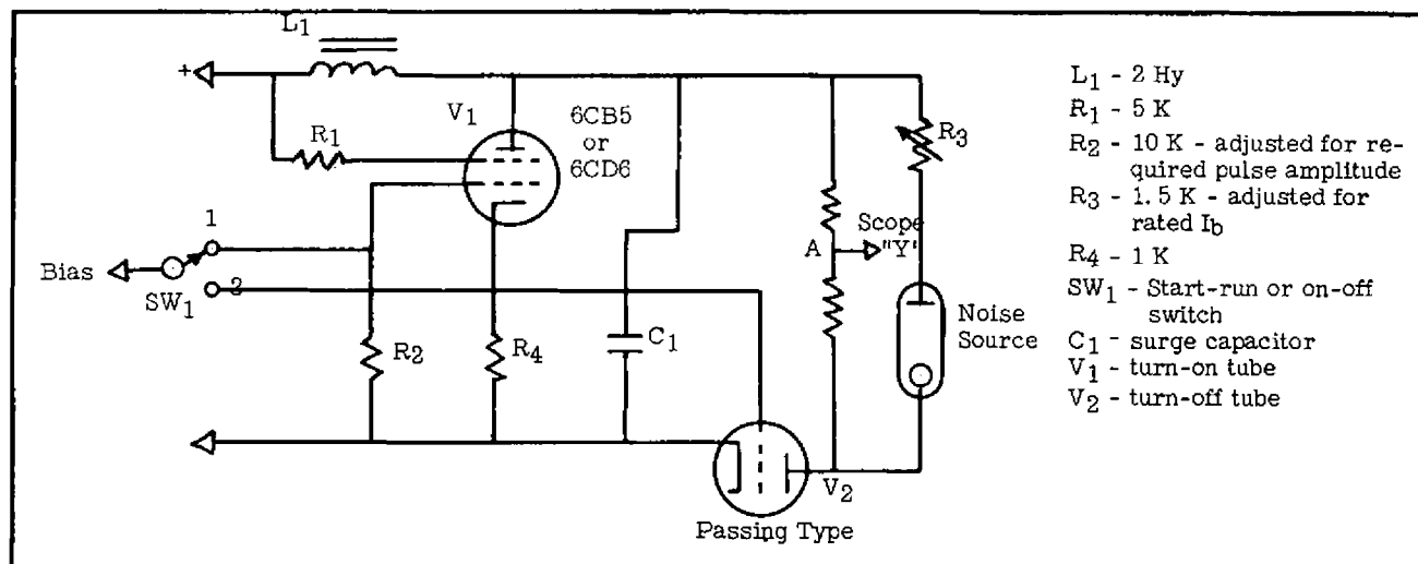
FIGURE 1: Typical Starting and Operating Circuit for Pulse Operation
