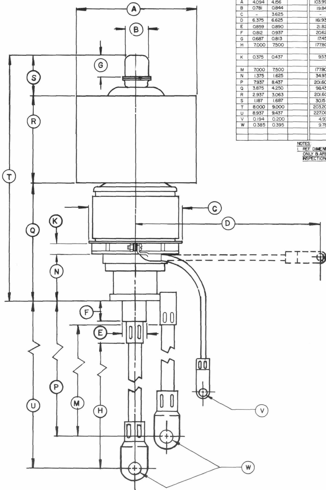
DIMENSIONAL DATA
