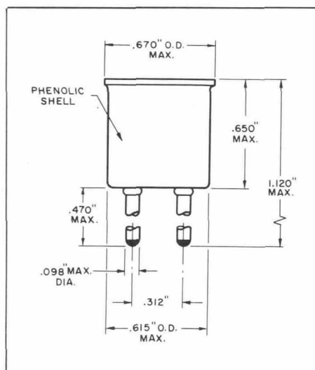
OUTLINE 8143-1
