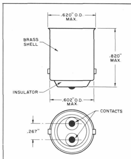
OUTLINE 8143-7
