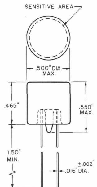
OUTLINE 8143
