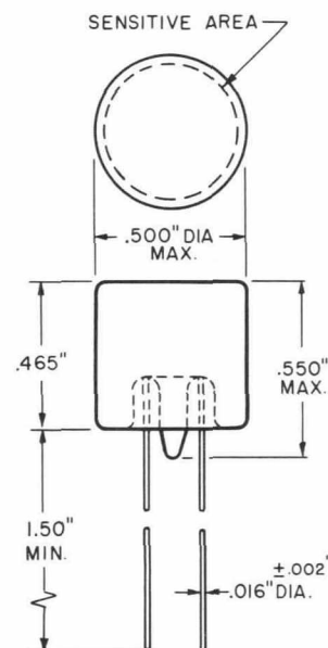
OUTLINE 8142
