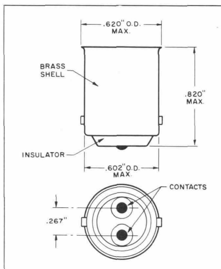
OUTLINE 8142-7
