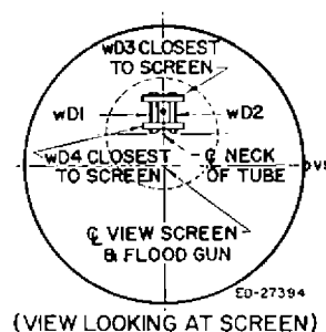
Figure 9 — Deflection Plate Orientation
