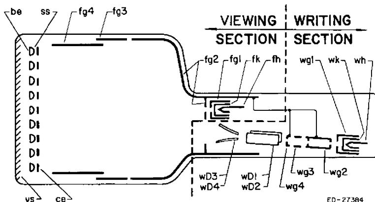
Figure 2 — Construction of Tube Shown Schematically
