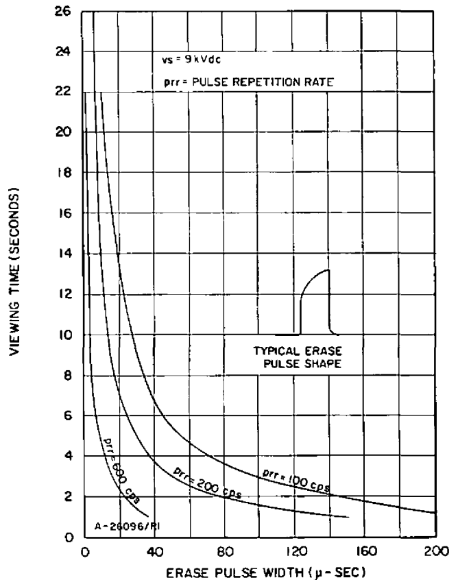
Figure 7 — Erase Characteristics
