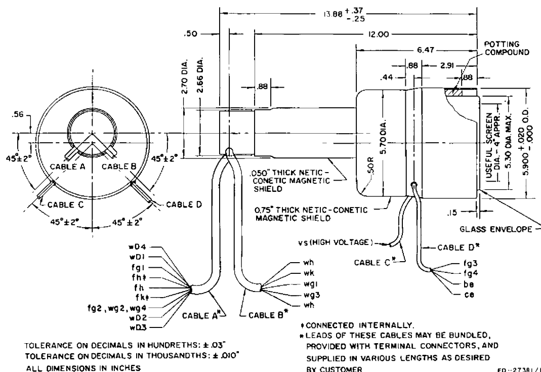
Figure 8 — Dimensions — ML-8130
