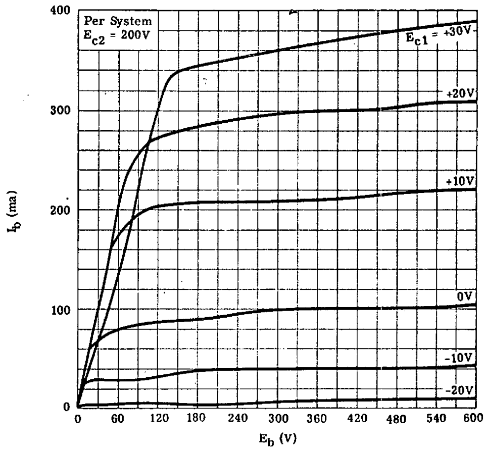
FIGURE 1. PLATE CHARACTERISTICS
