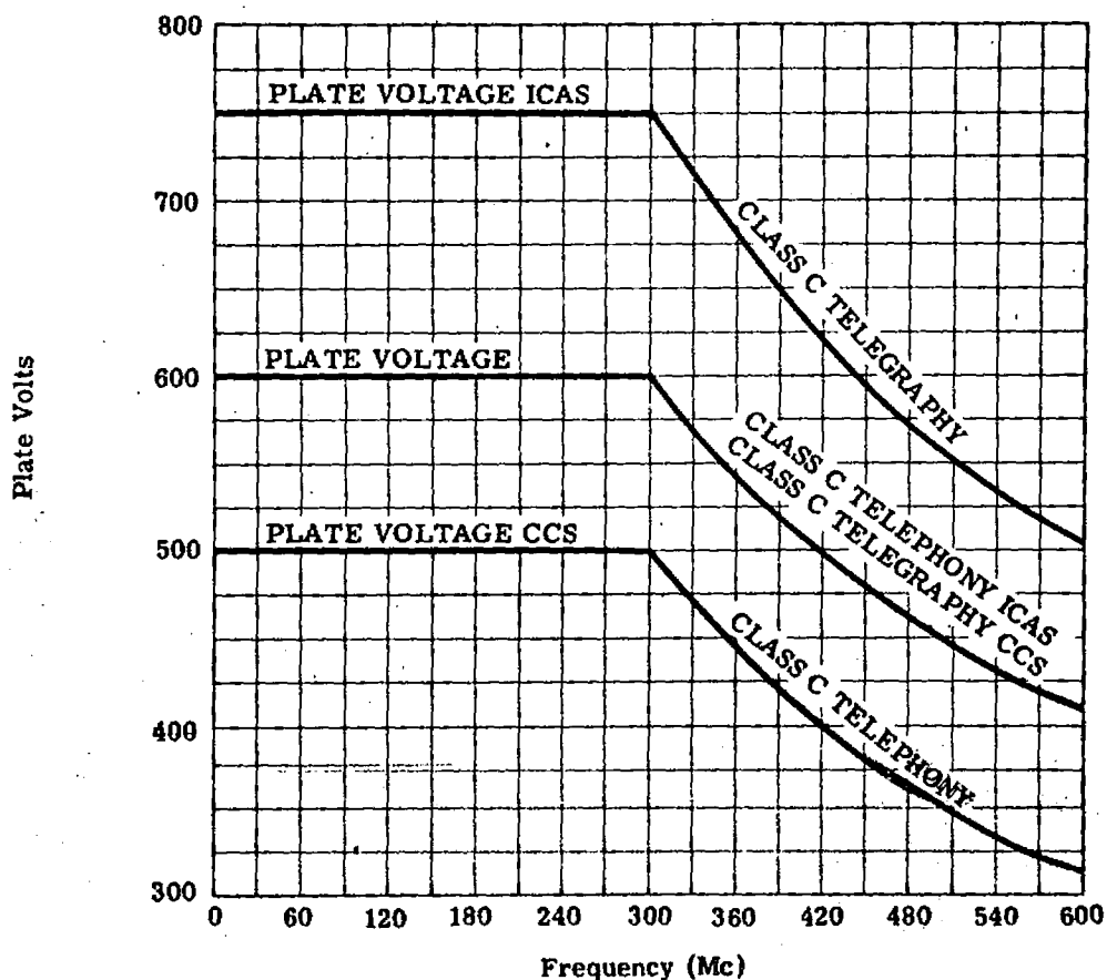
FIGURE 8. DERATING CURVES
