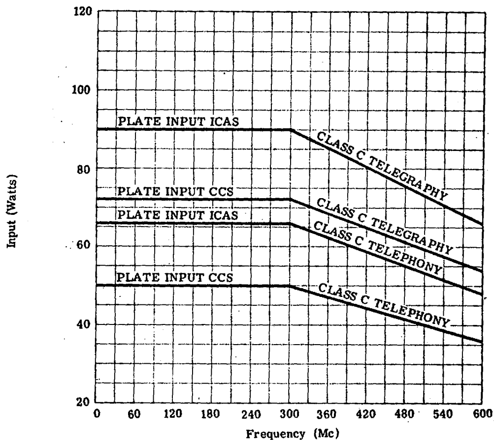
FIGURE 7. DERATING CURVES
