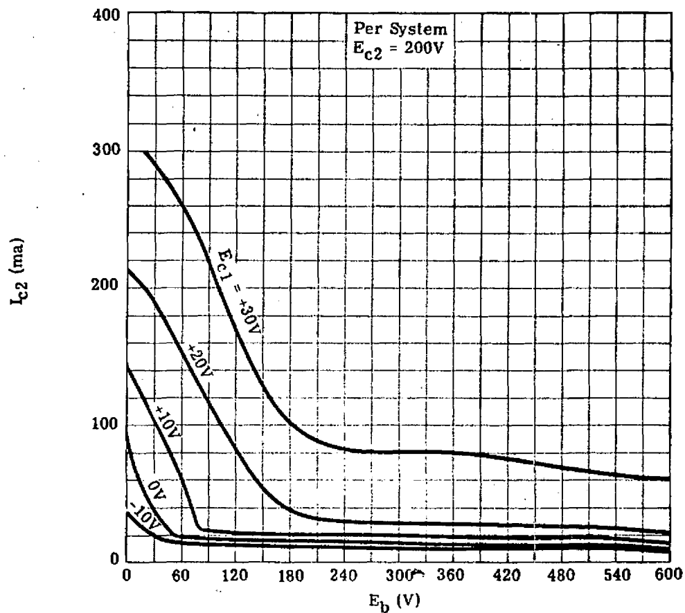
FIGURE 5. SCREEN GRID CHARACTERISTICS
