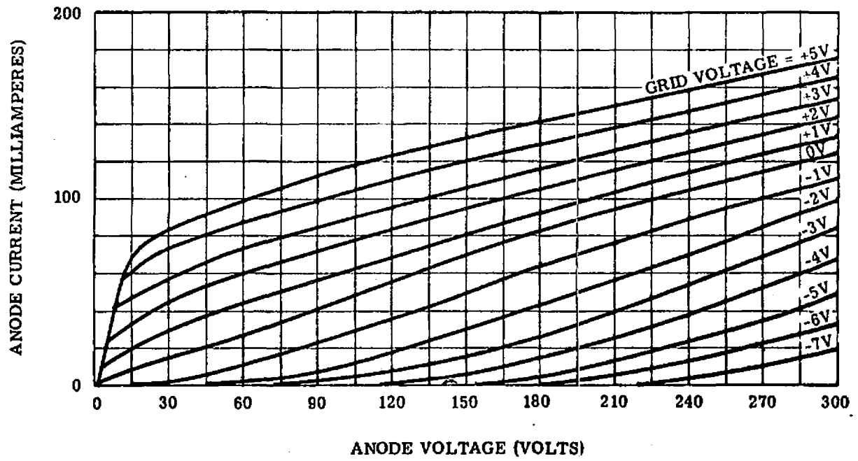
FIGURE 5. ANODE CHARACTERISTICS
