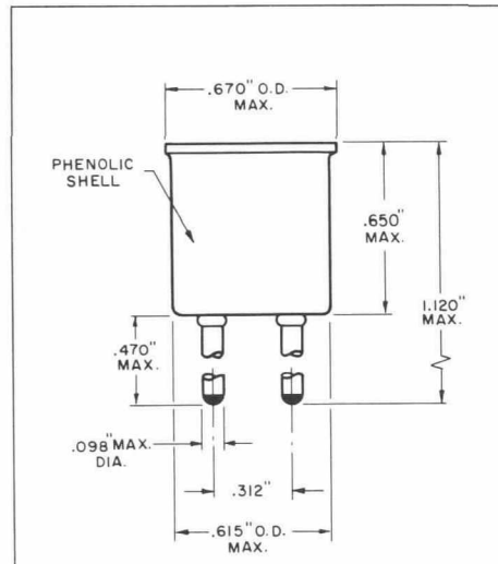
OUTLINE 8100-1
