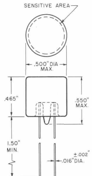
OUTLINE 8100
