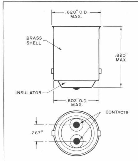
OUTLINE 8100-7
