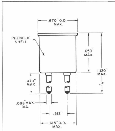
OUTLINE 8100-1
