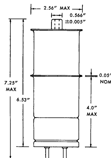
OUTLINE DRAWING
