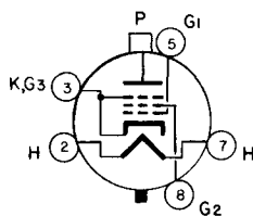
BOTTOM VIEW BASING DIAGRAM JEDEC 8LC
