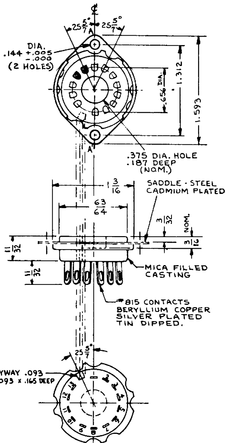
BOTTOM VIEW
