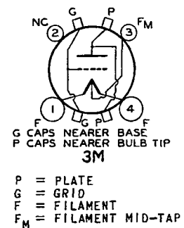
Bottom View of Socket Connections
