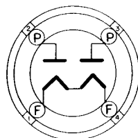
BOTTOM VIEW MEDIUM SHELL 4 PIN OCTAL BASE 4C
