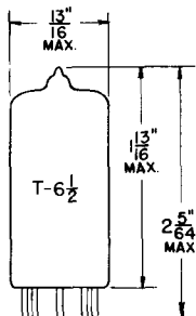
GLASS BULB
