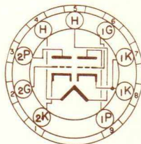
BOTTOM VIEW MINIATURE 9 PIN BASE
