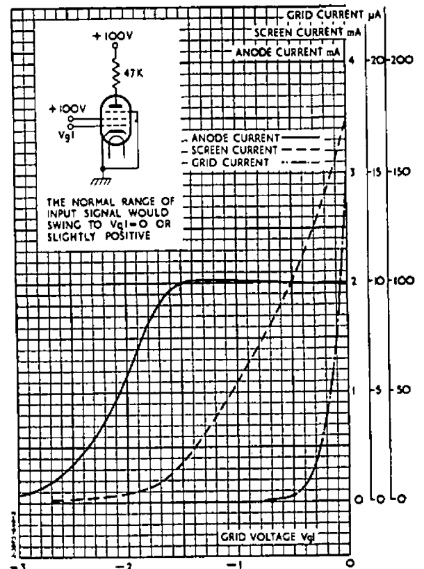
AVERAGE CHARACTERISTIC CURVES: I_a, I_{g2}, I_{g1}/V_g Used as a limiter in a synchronising separator circuit.
