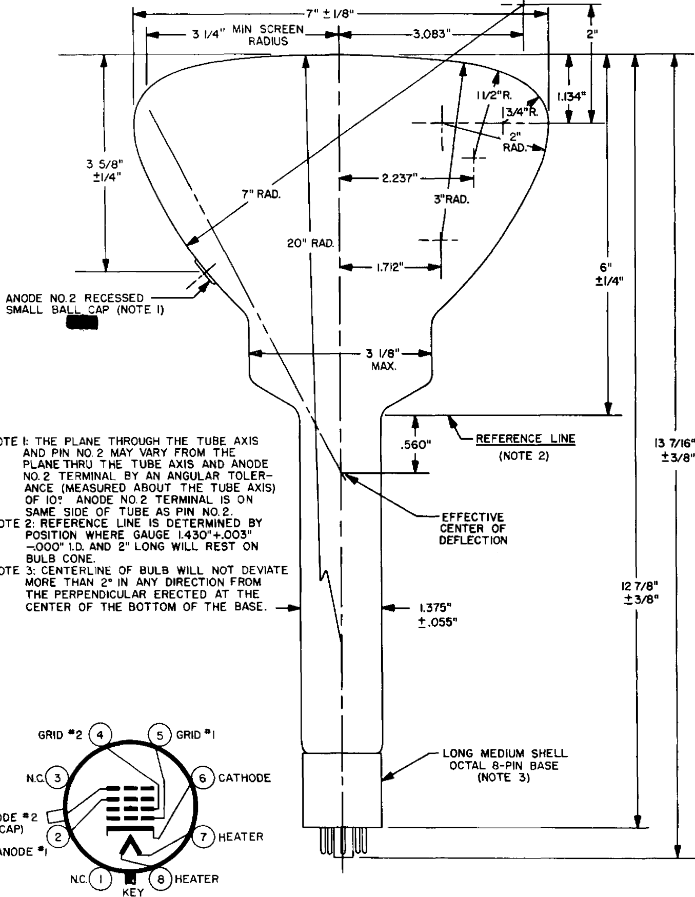
BASING DIAGRAM
