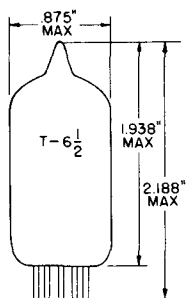
GLASS BULB SMALL BUTTON NOVAL 9 PIN BASE EP-1 OUTLINE DRAWING JEDEC 6-2
