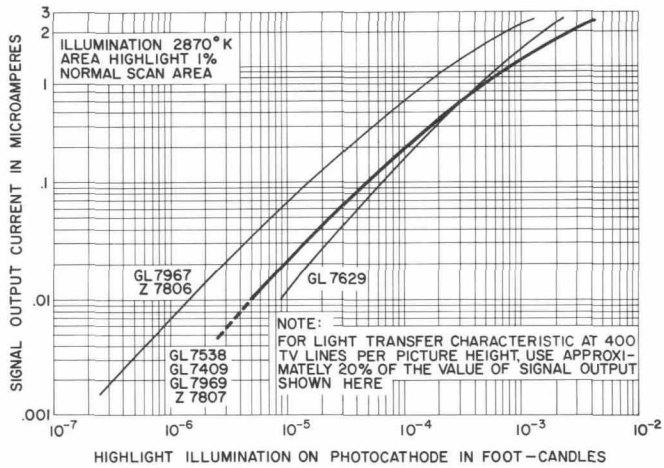
LIGHT TRANSFER CHARACTERISTICS
