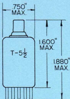
GLASS BULB 7 PIN MINIATURE OUTLINE DRAWING JEDEC E7-1
