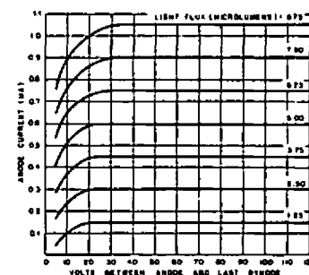
TENTATIVE AVERAGE ANODE CHARACTERISTIC VOLTS / STAGE - 145
