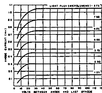
TENTATIVE AVERAGE ANODE CHARACTERISTIC
