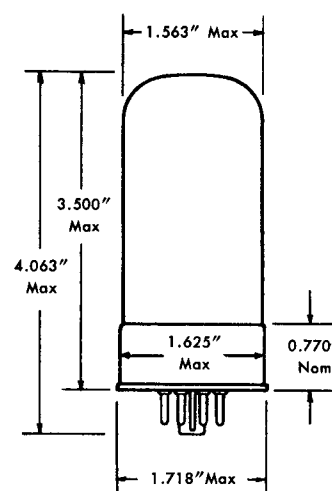
OUTLINE DRAWING
