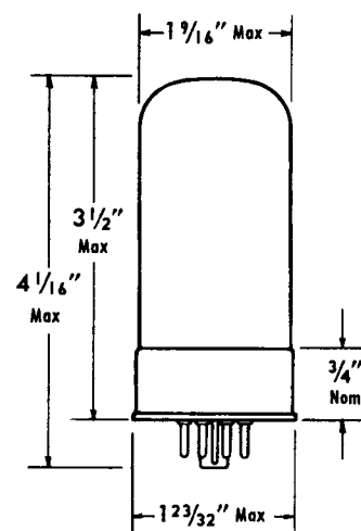
OUTLINE DRAWING
