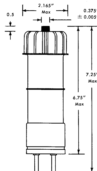
OUTLINE DRAWING
