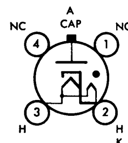
BASIC DIAGRAM BOTTOM VIEW
