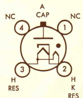
BASING DIAGRAM BOTTOM VIEW
