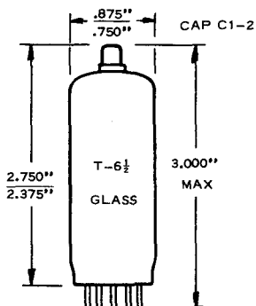
BUTTON 9 PIN MINIATURE BASE E9-1 GOLD PLATED PINS
