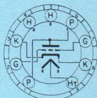
BOTTOM VIEW MINIATURE BUTTON 9 PIN BASE 9 MAX
