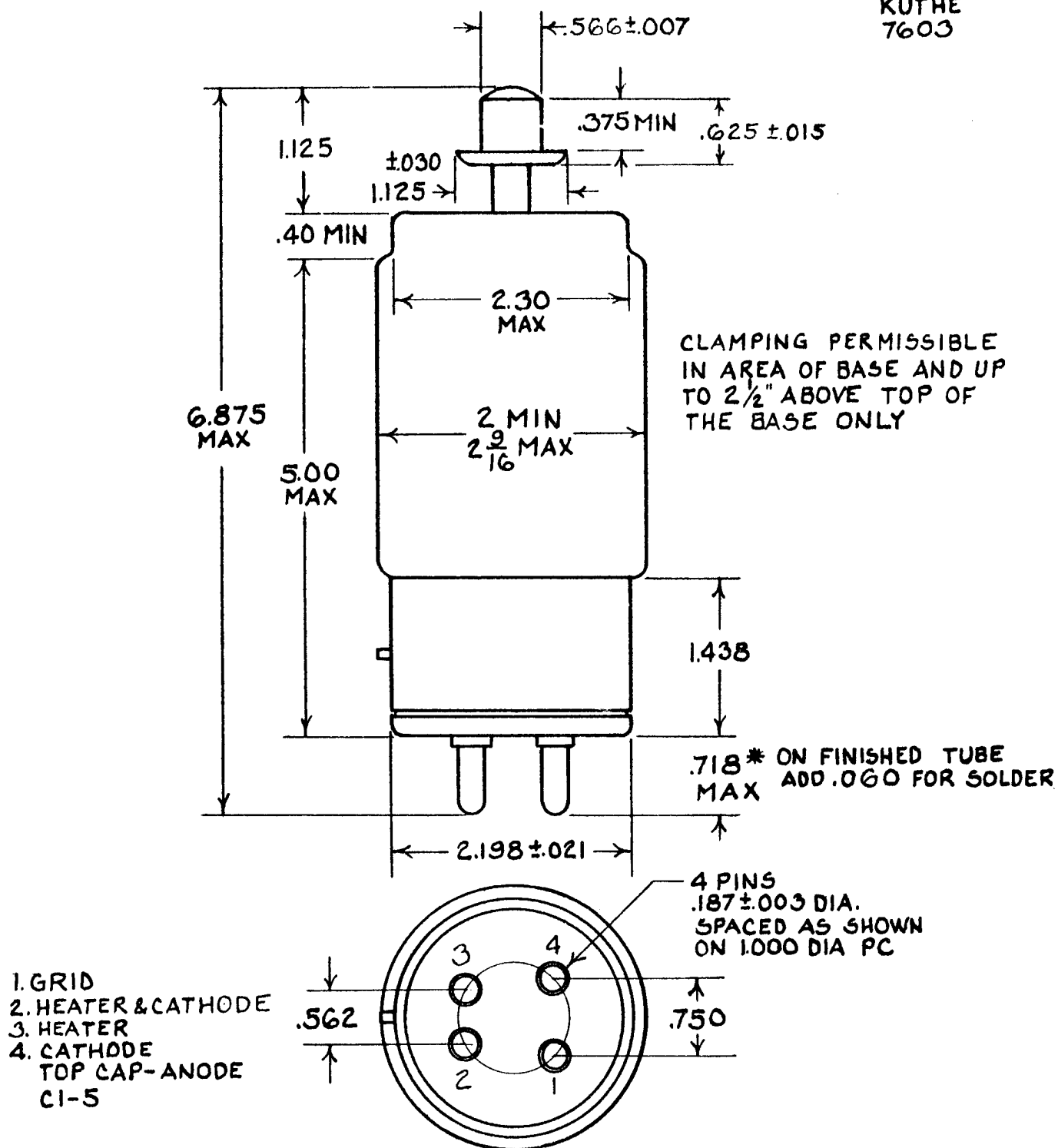
SUPER JUMBO 4-PIN WITH BAYONET A4-18 MIL-E-1D WITH CERAMIC INSERT
