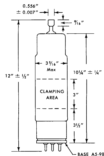
OUTLINE DRAWING
