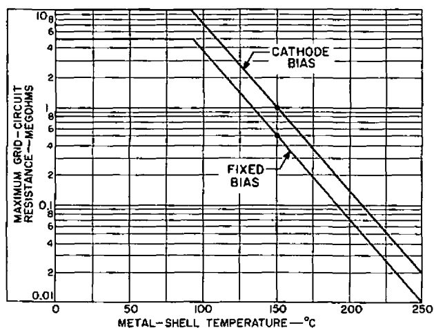
GRID-CIRCUIT-RESISTANCE RATING CHART
