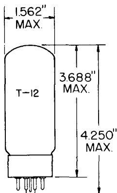
GLASS BULB SHORT MEDIUM SHELL 6 PIN OCTAL B6-148 LOW LOSS MATERIAL OUTLINE DRAWING JEDEC 17-15
