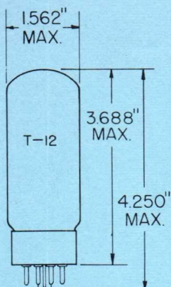
GLASS BULB SHORT MEDIUM SHELL 6 PIN OCTAL B6-148 LOW LOSS MATERIAL OUTLINE DRAWING JEDEC 12-15
