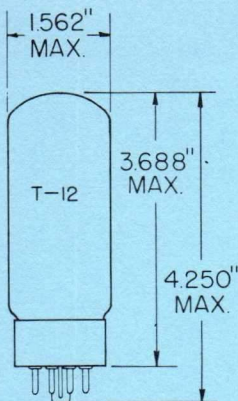
GLASS BULB SHORT MEDIUM SHELL 6 PIN OCTAL B6-248 LOW LOSS MATERIAL OUTLINE DRAWING JEDEC 12-15
